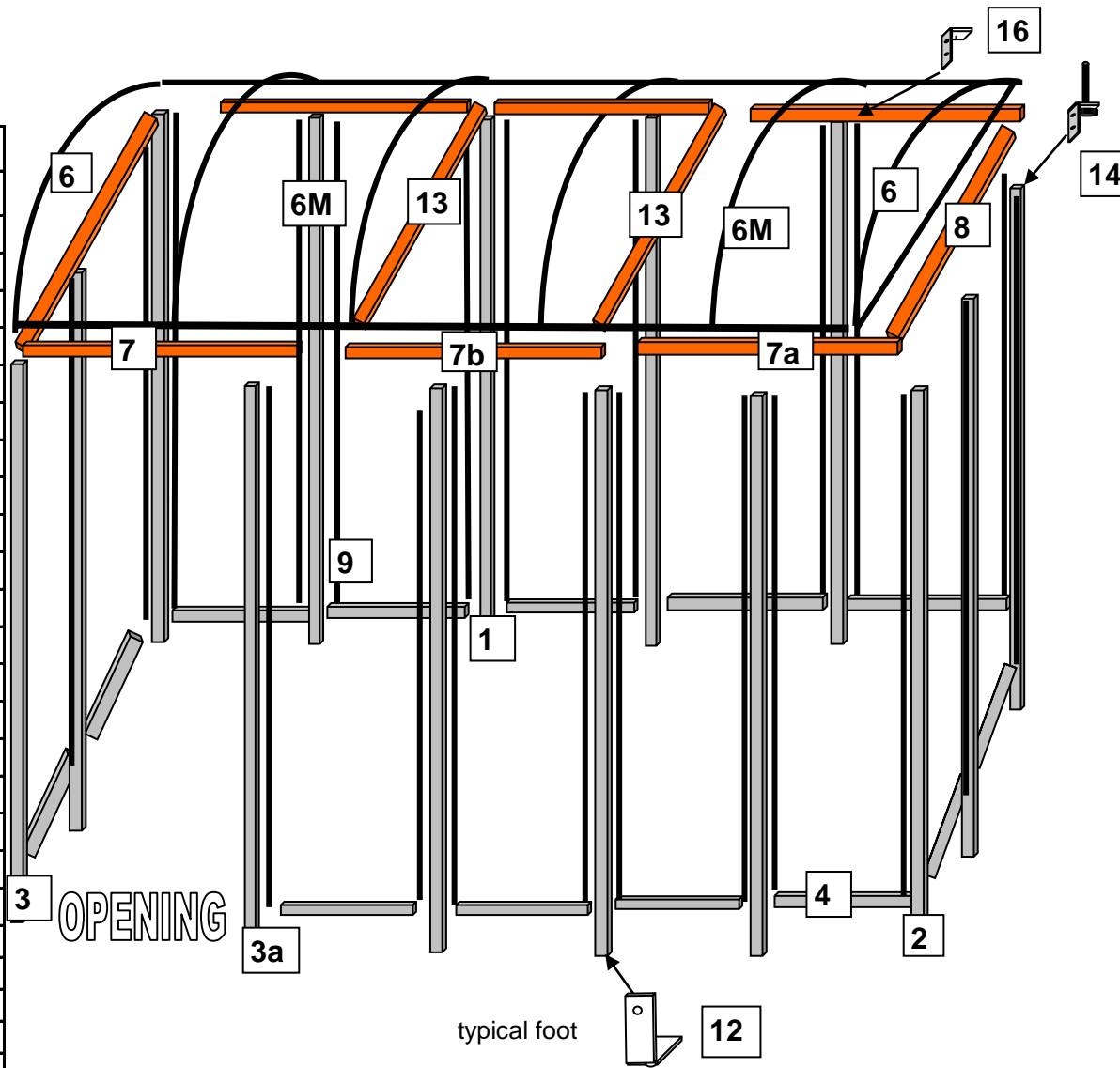
Layout of Uprights & Roof Fixing NBS0820FS
