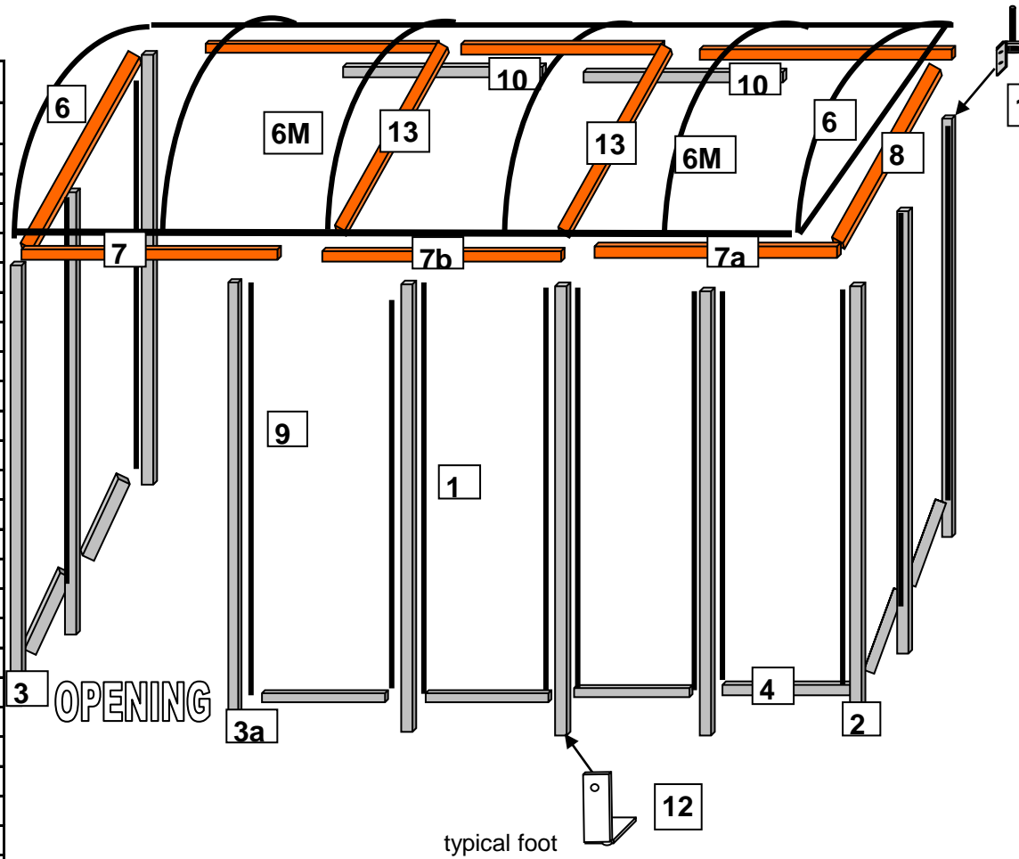
Layout of Uprights & Roof Fixing NBS0820BW
