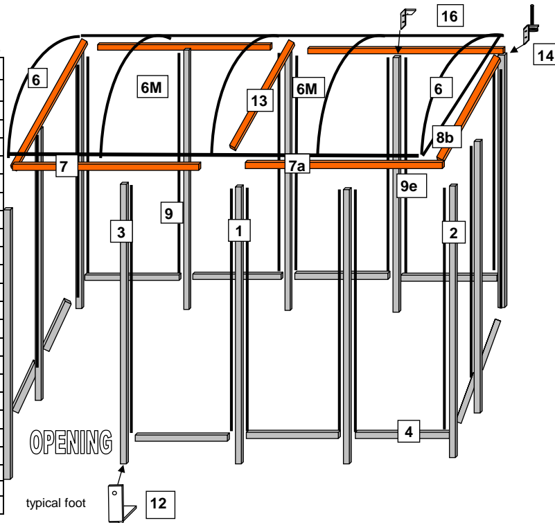
Layout of Uprights & Roof Fixing NBS0816FS
