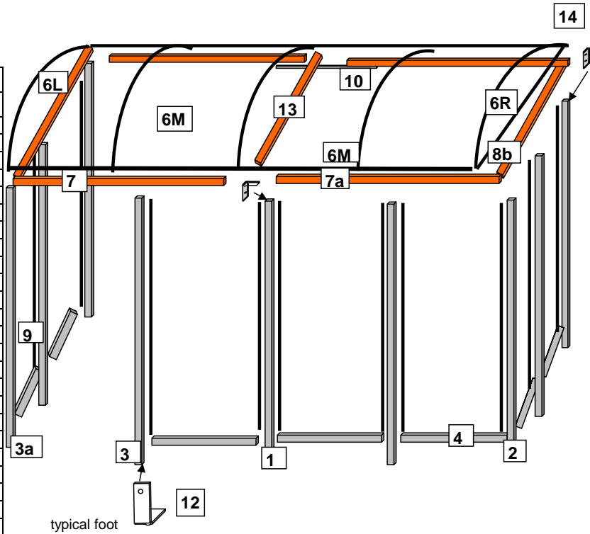
Layout of Uprights & Roof Fixing NBS0816BW
