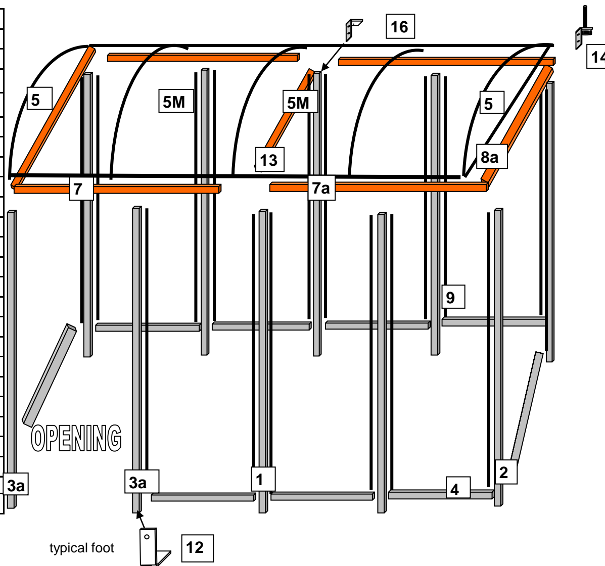
Layout of Uprights & Roof Fixing NBS0416FS
